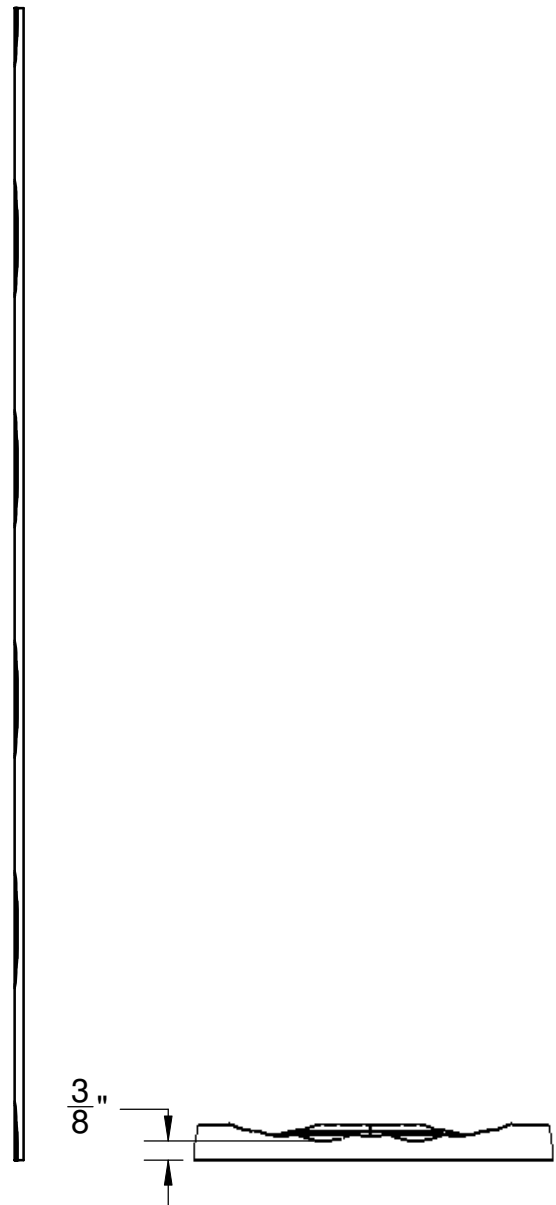
DETAIL A SCALE 1 : 4
