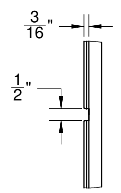
DETAIL A SCALE 1 : 4
