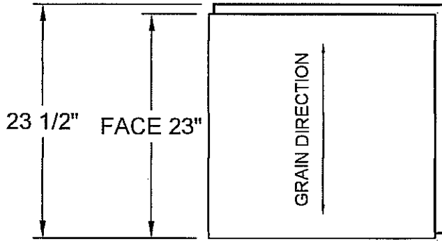
Typical Panel
