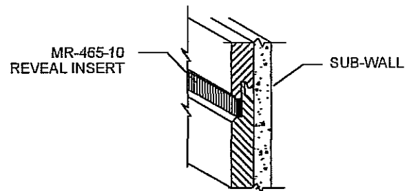
PANELS WITH 1/4" REVEAL ONLY
