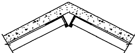
Other than 90 degrees inside corner
