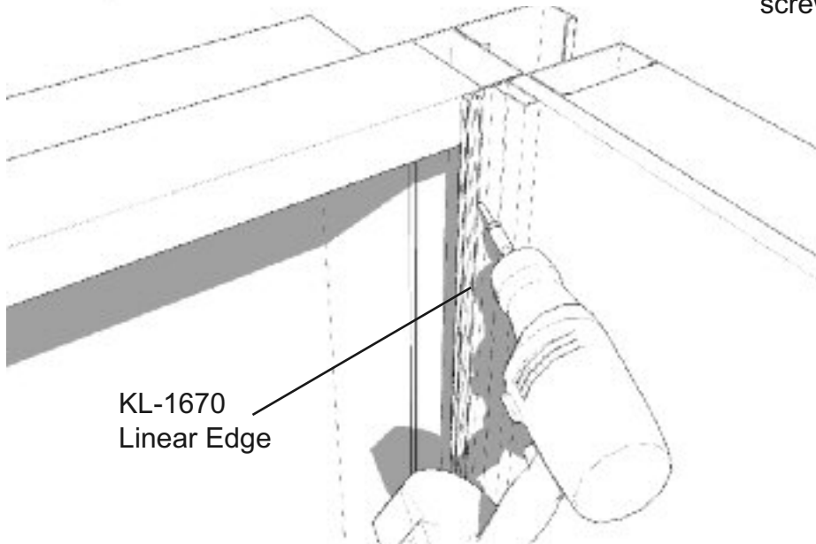
Detail of vertical trim attachments.
