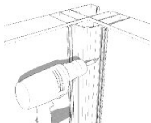
Detail of vertical trim attachments.
